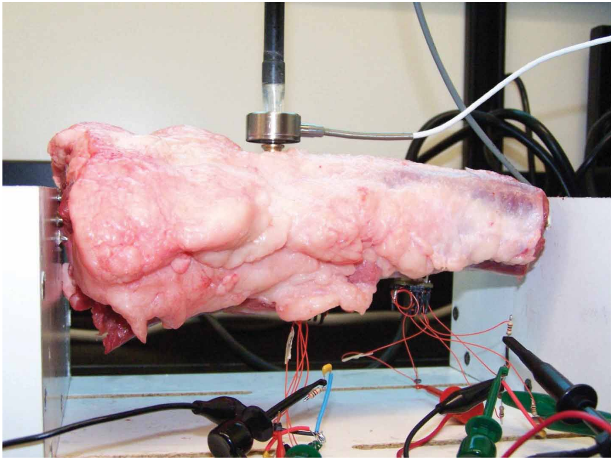
FIGURE 2. Impacted mechanics set-up. 100 lb load cell is attached to cleaned section of central vertebrae [five in total] and aligned with stylus of device. Three-dimensional accelerometer on central vertebrae [bottom] measures stylus effects on in situ vertebrae.
